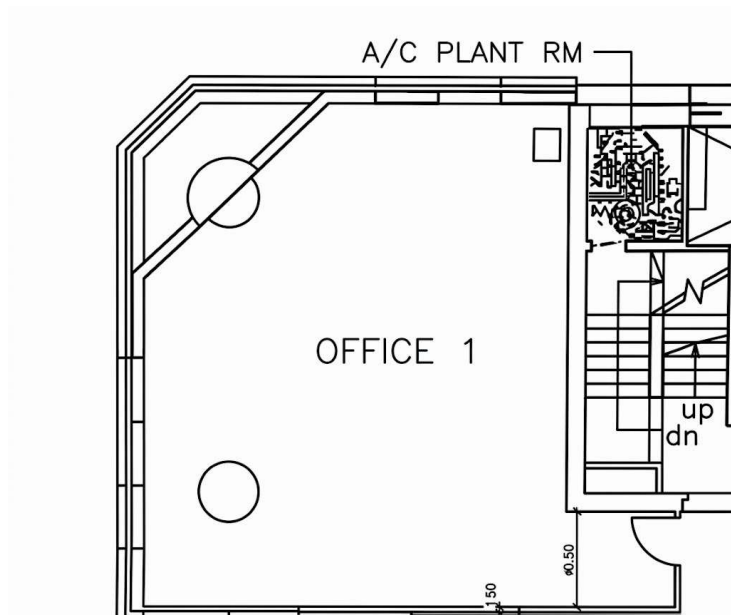
Unit 1 of 23/F Floor Plan For Identification Only
