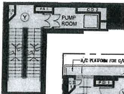
HALF LANDING PART PLAN
