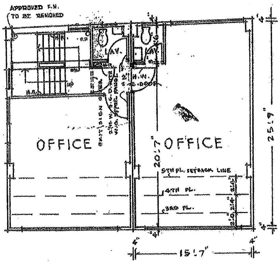
1ST - 5TH FLOOR PLAN
