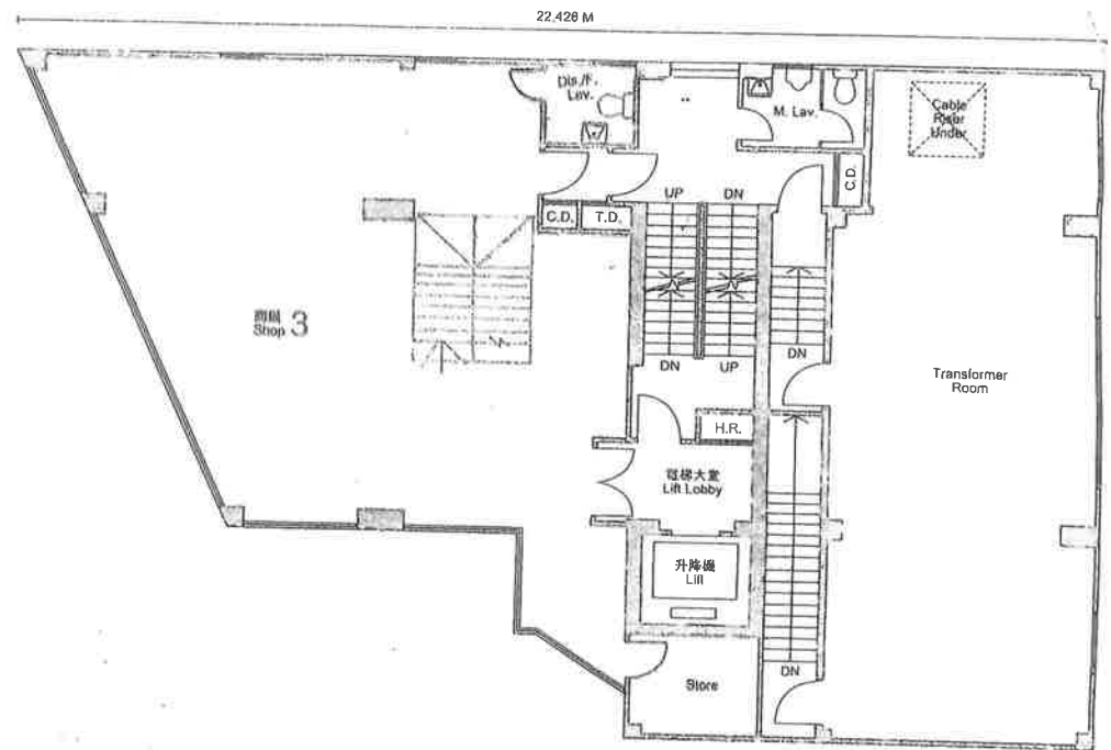
一樓平面圖 First Floor Plan
